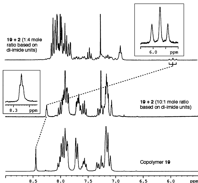
Figure 10. 1 H NMR spectra (250 MHz) showing the consequences of increasing the proportion of tweezer molecule 2 relative to the pyromellitimide content of copolymer 19 .
