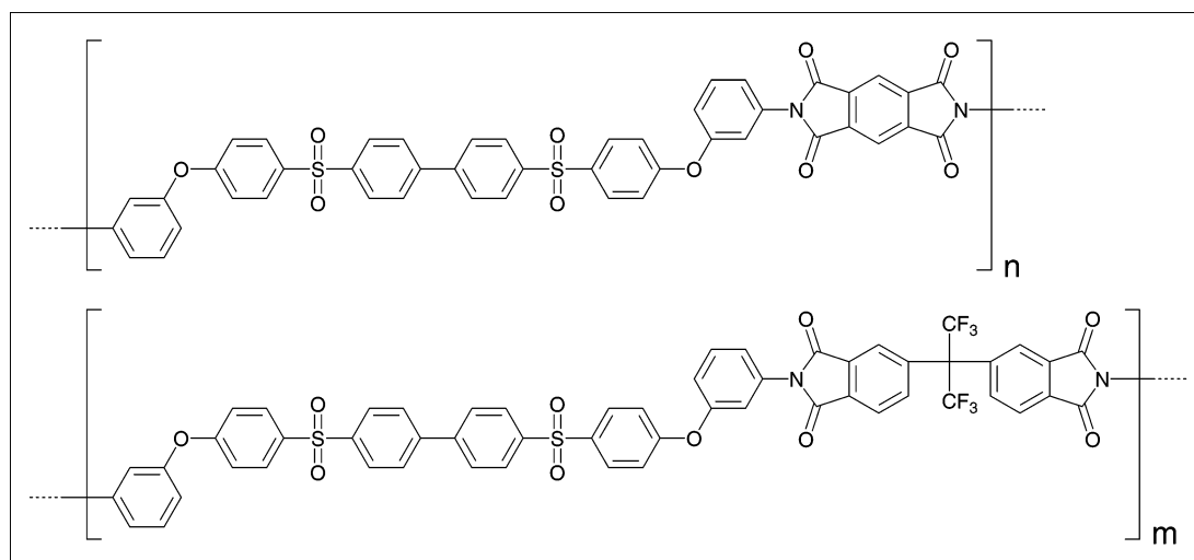
Chart 6. Copolyimides Derived from Hexafluoroisopropylidene-diphthalic Dianhydride.
