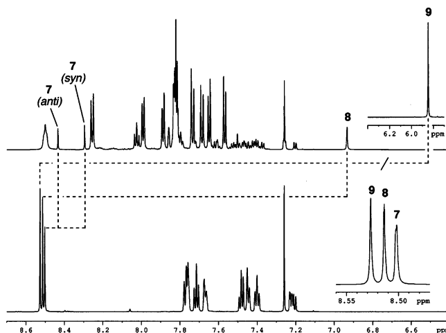
Figure 6. The 700 MHz 1 H NMR spectra (CDCl 3 /(CF 3 ) 2 CHOH, 6:1 v/v) of a 1:1:1 mixture of the doubly hindered, singly hindered, and unhindered diimides 7 , 8 , and 9 , respectively (lower trace), and the same mixture in the presence of a fourfold molar excess of 3 (upper trace). Complexation shifts of the pyromellitimide protons are highlighted.
