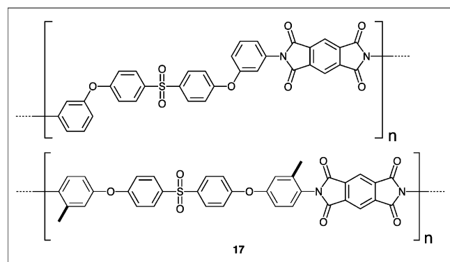
Chart 5. Polyimides Derived from Short-Chain, Nonfolding Diamines a
