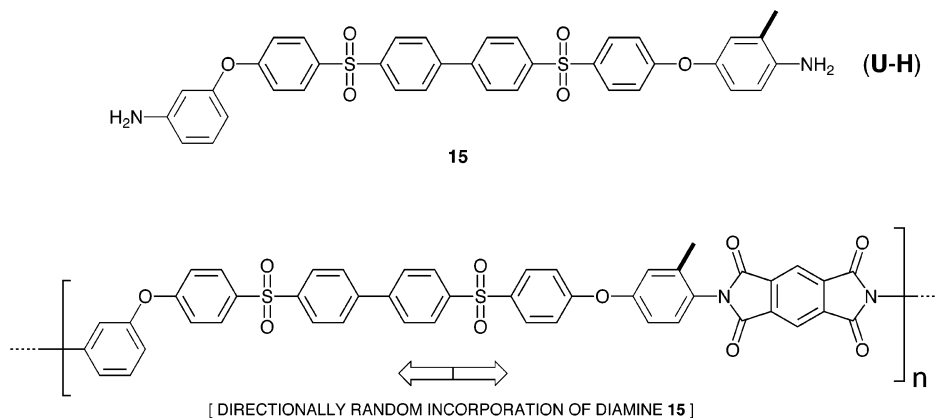
Chart 4. An Unsymmetrical Diamine and Its Directionally-Random Polyimide a
