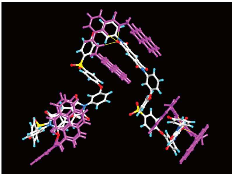
Figure 9. Energy-minimized model for adjacent binding of three tweezer molecules to consecutive pyromellitimide residues in the nonfolding poly(ether-imide-sulfone) 17 (Chart 5). Hydrogen bonds (N–H···O and C–H···O) between the tweezers and the polymer chain are shown in yellow.
